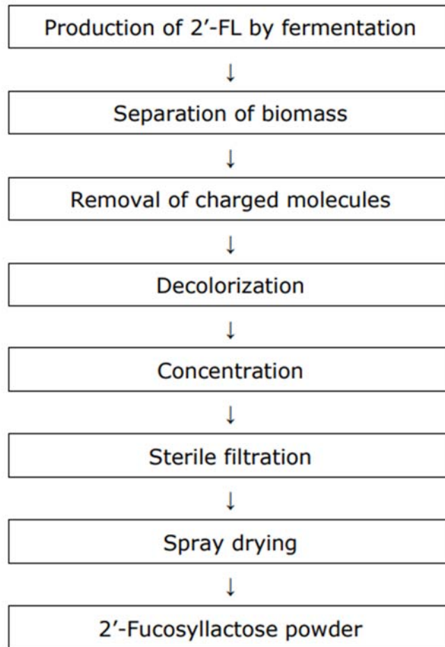
Figure 2.2 Purification process for 2'-FL micro
