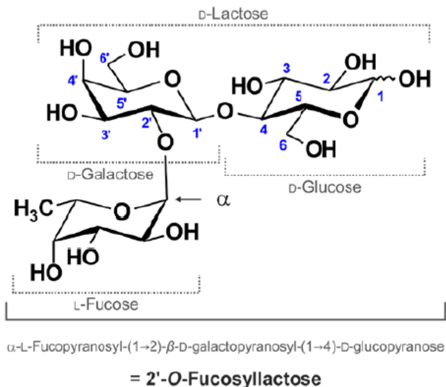
Figure 2.1 Molecular Structure of 2'-FL (Image from: EFSA NDA Panel 2015 3 )
